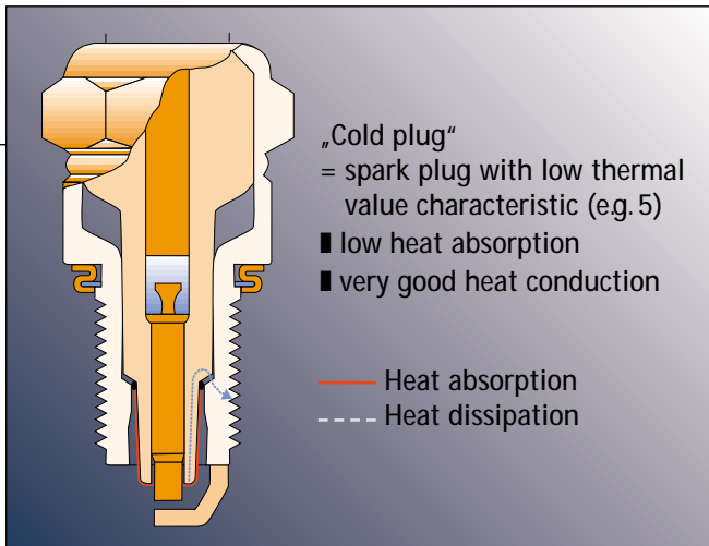
Cold spark plug
